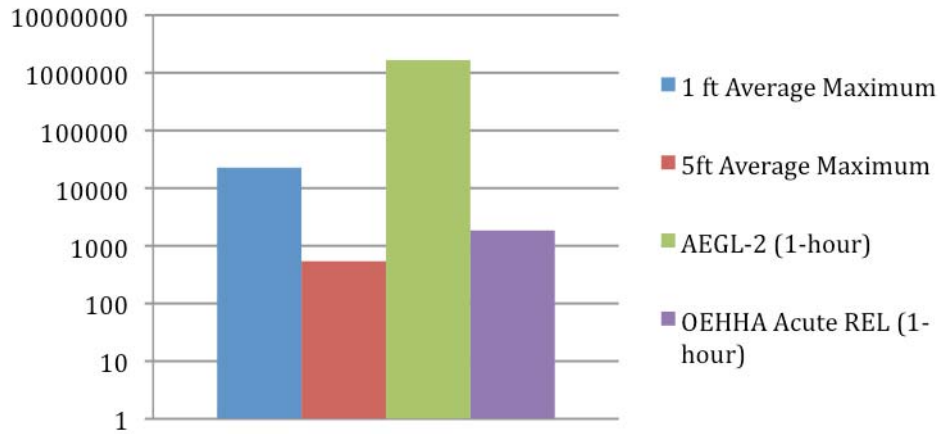
Figure 2. The maximum mercury vapor concentrations at 1ft and 5 ft from floor (average of three trials).
