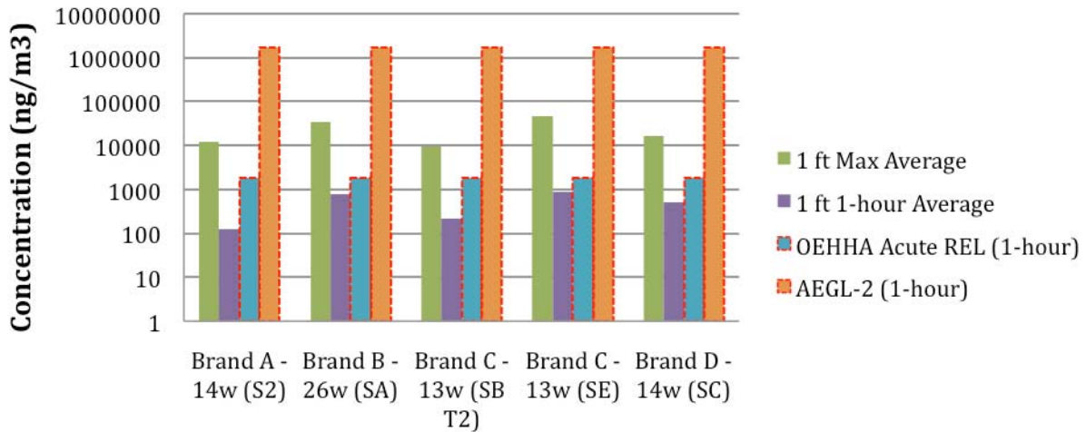
Figure 4. Comparison of maximum and 1-hour average mercury concentrations at one foot from scenarios that tested a variety of CFL Brands and Wattages.
