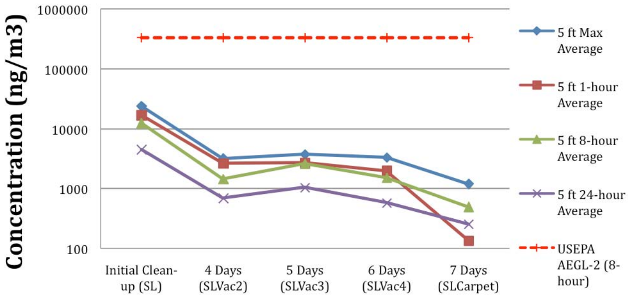
Figure 6. Mercury concentrations at 5 feet from a scenario (SL) with multiple vacuuming sessions over a seven-day period.
