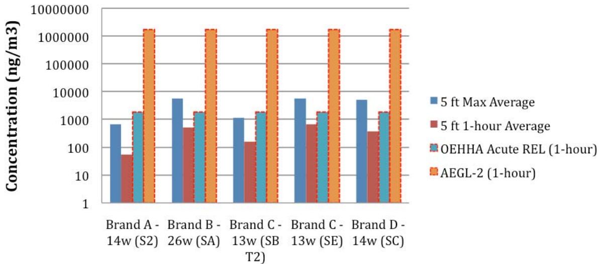
Figure 5. Comparison of maximum and 1-hour average mercury concentrations at five feet from scenarios that tested a variety of CFL Brands and Wattages.
