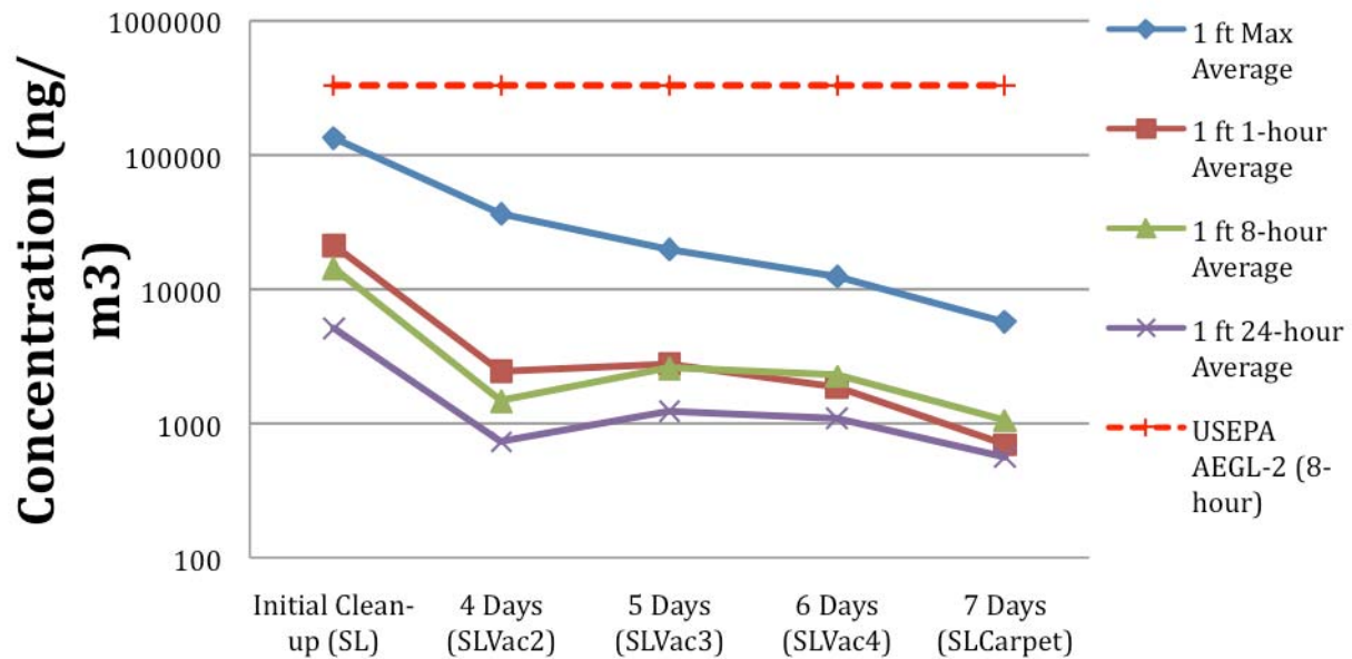
Figure 7. Mercury concentrations at 1 foot from a scenario (SL) with multiple vacuuming sessions over a seven-day period.
